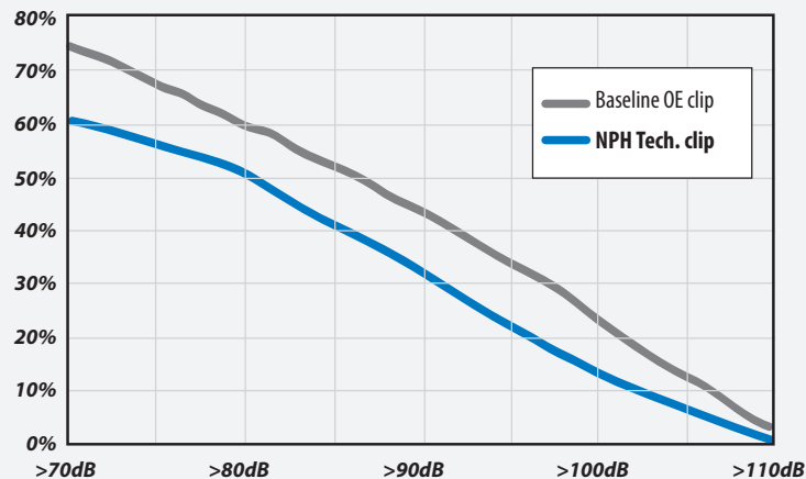
Abutment Clip Comparison – Percent Noise at Specified dB levels from SAE J2521 Noise Dyno test on W-body Front Brake
